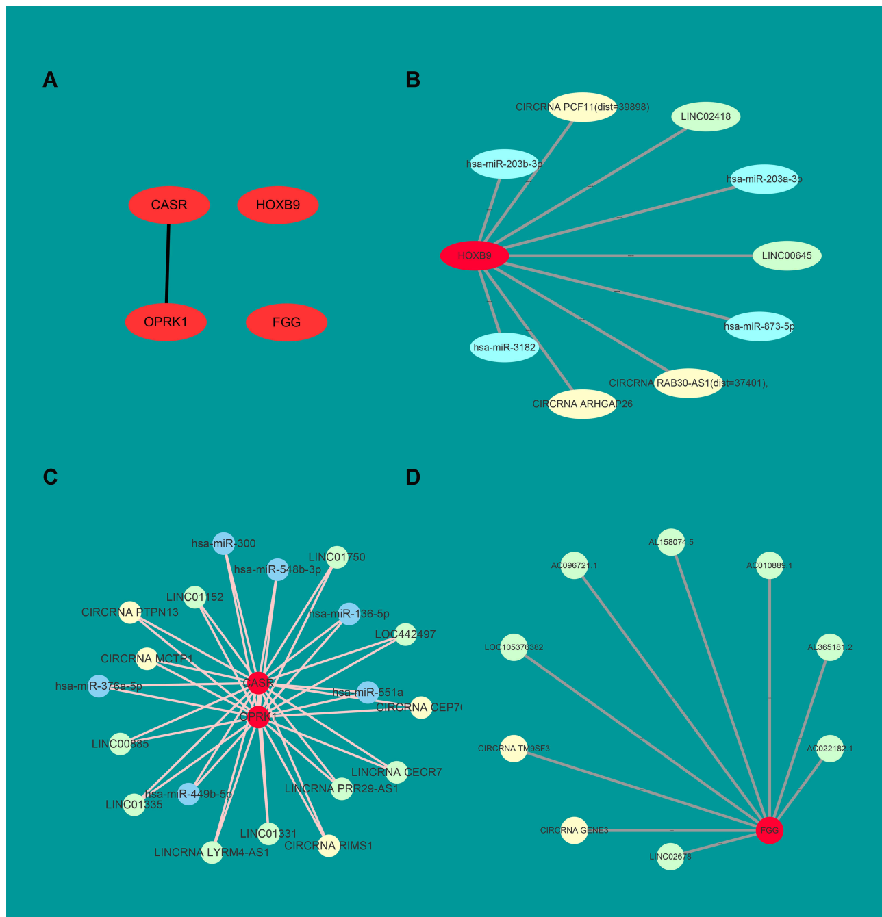
Figure 4 OPRK1 , CASR , HOXB9 and FGG are the hub genes in the PPI network. (A) The top four hub genes OPRK1 , CASR , HOXB9 and FGG . The hub genes were screened out by the cytohubba-APP in the Cytoscape. The top four hub genes degree score are all equal to 3. (B) In the network, taking HOXB9 as the hub gene, its related lincRNAs, circRNAs and miRNAs. (C) OPRK1 and CASR genes related RNAs. (D) FGG and its related RNAs. Red circles represent hub mRNAs. The green circles represent lincRNA, the blue circles represent miRNA and the yellow circles represent circRNA.
