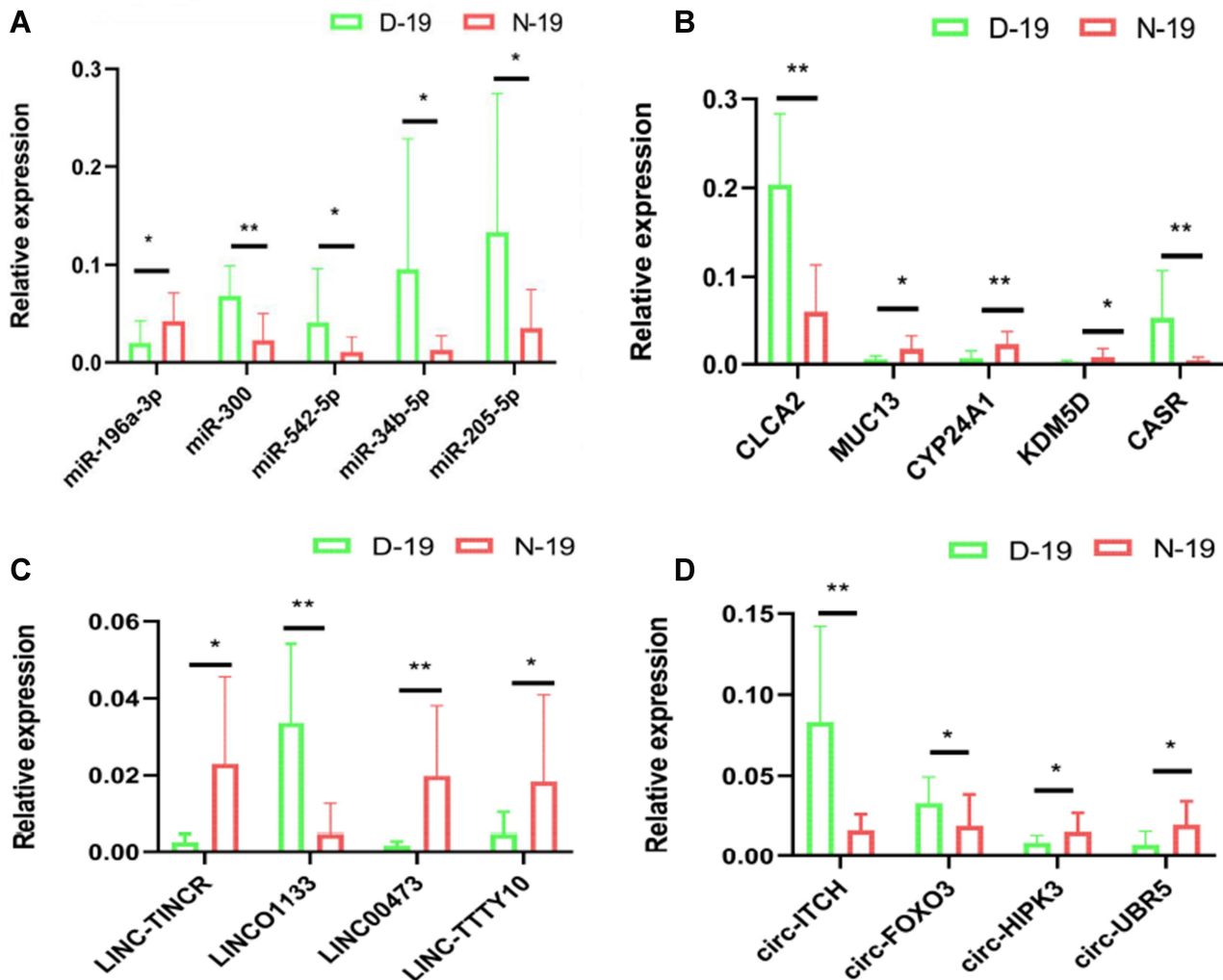
Figure 6 RT-qPCR of the DERNAs, * p < 0.05 , ** p < 0.01 . D-19 indicate EGFR-19-D, N-19 indicate EGFR-19 wild-type. (A) Relative expression of 5 miRNAs between D-19 and N-19 groups. (B) Relative expression of five mRNAs between D-19 and N-19 groups. (C) Relative expression of four lncRNAs between D-19 and N-19 groups. (D) Relative expression of four circRNAs between D-19 and N-19 groups.
