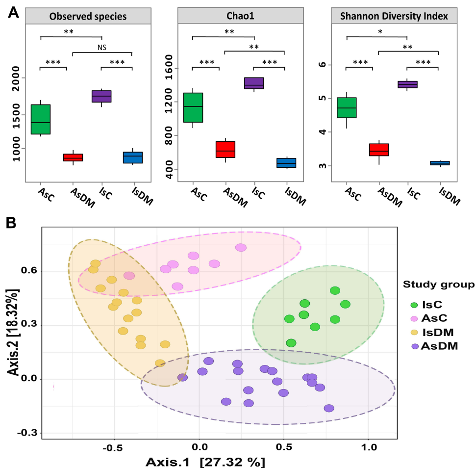
Figure 2 Diversity analyses of gut microbiomes. (A) Bacterial alpha diversity indices were represented by box plots of the following indices: the number of observed species Chao1 index and Shannon diversity index. X-axis represented the study groups, while alpha indices were plotted on the Y-axis. The median was represented by the line in each box, the interquartile range (IQR) between the 25th and 75th percentile was delimited by the box, and the range was outlined by the whisker. The nonparametric Wilcoxon rank-sum test was used to define the statistical significance of pairwise comparisons. Significant differences were displayed with either NS ( P > 0.05 ), * ( P < 0.05 ), ** ( P < 0.01 ) or *** ( P < 0.001 ). (B) Principal coordinates analysis (PCoA) of gut microbiomes based on weighted UniFrac distance matrices. PCoA plot represented the similarity distances between gut microbiota of healthy and diseased groups. The significant clustering was denoted by ellipses (Adonis: r^2 = 0.047 , P = 0.00092 ).
