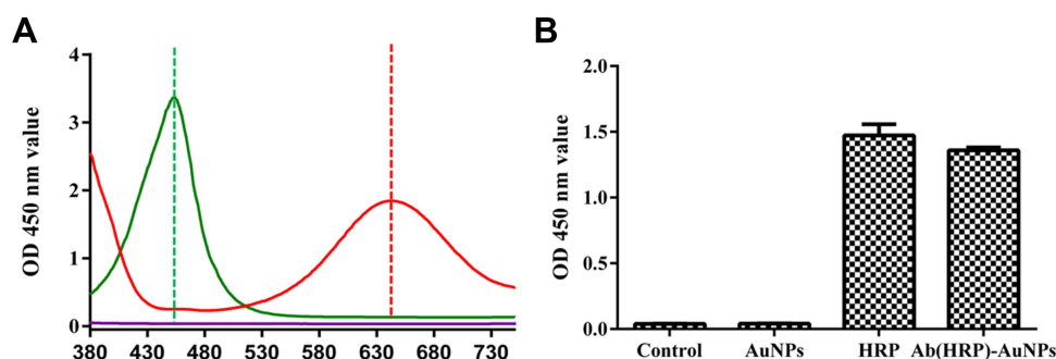
Figure 2 Confirmation of the catalytic function of Ab (HRP)-AuNPs complex. (A) The color reaction of TMB catalyzed by the Ab (HRP)-AuNPs complex in the presence of H_2O_2 (the purple line is the absorption spectrum of the reaction solution without the presence of Ab (HRP)-AuNPs complex; the red and green line are the absorption spectra of the reaction solution mixed with Ab (HRP)-AuNPs complex before and after addition of H_2SO_4 respectively). (B) Comparison of the catalytic activity of 0.95 nM pure AuNPs, 1.09 \mu\text{g/mL} pure HRP and Ab (HRP)-AuNPs complex (prepared from 0.95 nM AuNPs and 1.09 \mu\text{g/mL} HRP).
