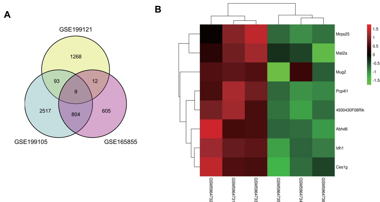
Figure 4 Identification of DEGs in NAFLD mouse model based on bioinformatics analysis. (A) Venn diagram for overlapping DEGs of the liver tissues among control and NAFLD group from the three cohort profile sets (GSE199121, GSE199105, GSE165855). (B) A Heatmap of DEGs between the normal and NAFLD group from the GSE199121 dataset, where DEGs overlapped with the other two datasets. Normal group was GSM5964731, GSM5964732 and GSM5964733; NAFLD group was GSM5964734, GSM5964735 and GSM5964736. Statistically significant DEGs were defined based on gene upregulation FC > 1 and P < 0.1 as the cut-off criteria.
