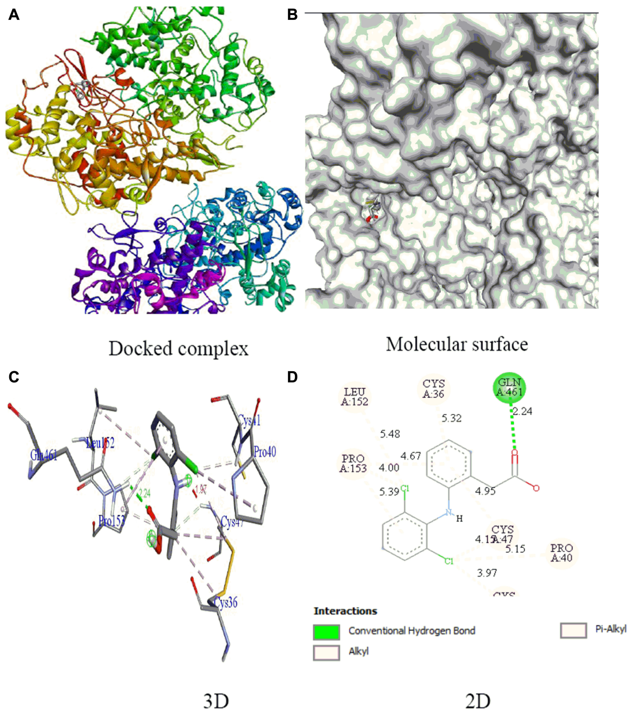
Figure 5 The binding of diclofenac with ICX2 protein complex: (A) Docking complex; (B) Molecular surface; (C) 3D interaction; (D) 2D interaction.
