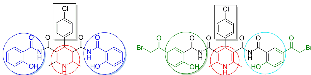
Figure 3 Structure–activity relationship of compounds 2c and 3c.
