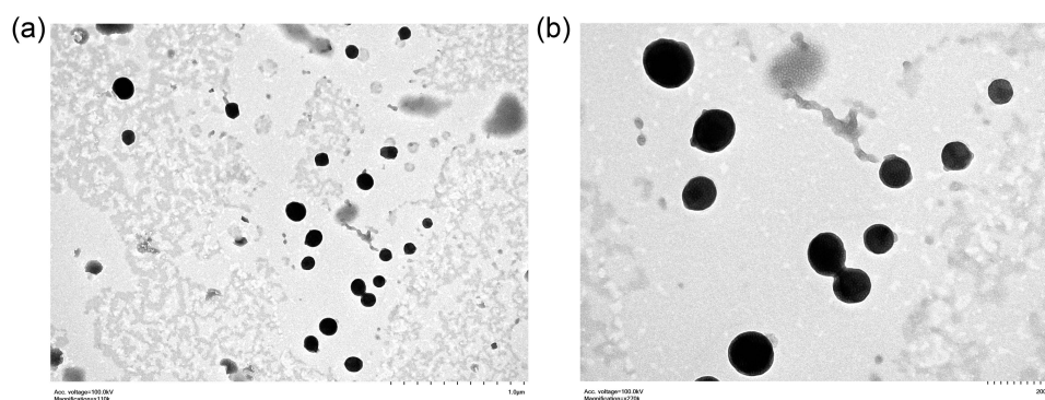
Figure 3 Transmission electron microscopy of SNEDDS. (a) Magnification: \times 110\text{k} , (b) magnification \times 270\text{k} .
