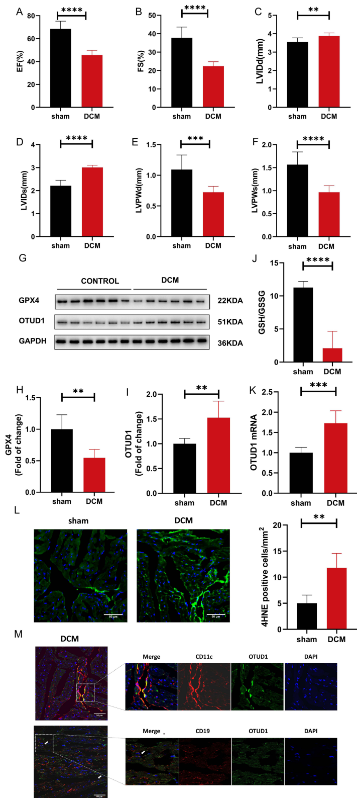
Figure 7 The verification of OTUD1 in the heart of DCM mice. (A-F) Cardiac systolic function index ( n=10 in each group); (G-I) representative WB bands and quantification of relative protein expression for GPX4 and OTUD1 ( n=6 in each group); (J) the GSH/GSSG ratio of sham and DCM mouse heart ( n=6 in each group); (K) the expression level of OTUD1 mRNA in the heart of DCM mouse ( n=6 in each group). (L) Representative image of 4-hydroxynonenal staining in sham and DCM mouse hearts; (M) colocalization between OTUD1 and CD11c and CD19 were analyzed by immunostaining in DCM mouse hearts. Data are shown as mean \pm SD and were analyzed by a two-tailed unpaired t -test Ejection fraction (EF); shortening fraction (FS), left ventricular posterior wall systolic thickness (LVPWs); left ventricular posterior wall diastolic thickness (LVPWd); left ventricular systolic internal diameter (LVIDs); left ventricular diastolic internal diameter (LVIDd). ** p < 0.01 , *** p < 0.001 and **** p < 0.0001 .
