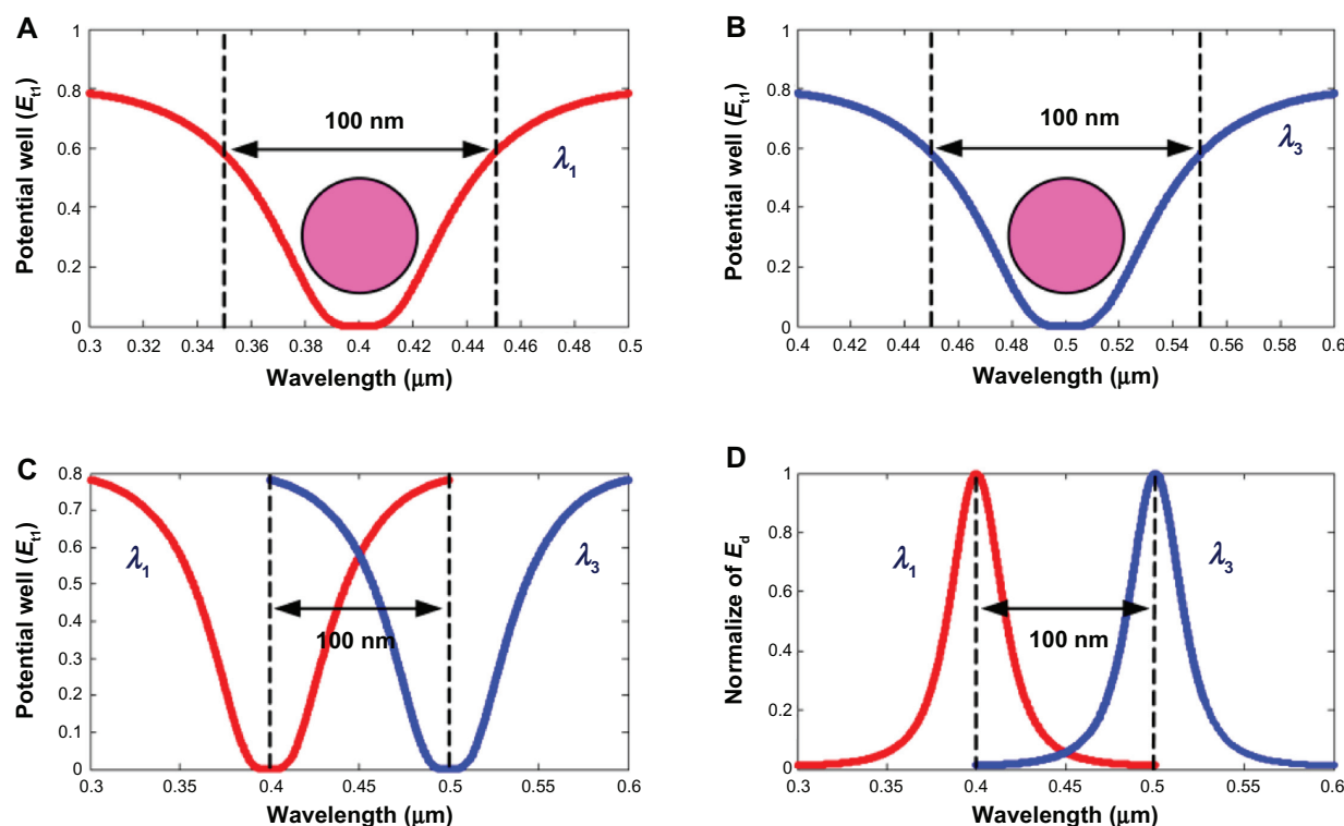
Figure 5 Results of the trapping tools, where A and B show different sizes and wavelengths, C shows tweezer separation, and D shows normalized tweezers, where R_{\text{in}} = 20 \mu\text{m} , R_R = R_L = 5 \mu\text{m} . The coupling coefficients are \kappa_0 = 0.5 , \kappa_1 = 0.35 , \kappa_2 = 0.1 , and \kappa_3 = 0.35 . The input power is 1 VV, R_{\text{in}} = 20 \mu\text{m} , R_L = R_R = 5 \mu\text{m} , ( A ) wavelength = 400 nm, ( B ) wavelength = 500 nm, ( C ) wavelengths = 400, 500 nm at through port, ( D ) wavelengths = 400, 500 nm at drop port.
