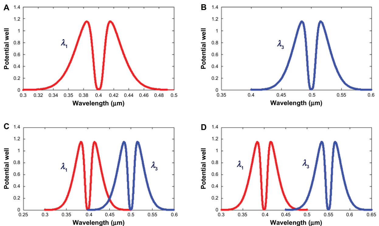
Figure 4 Result of the dynamic tweezers with different wavelengths (A–D), showing the tunable tweezer by coupling constants, where R_{ad} = 20 \mu\text{m} , R_R = R_L = 5 \mu\text{m} .
