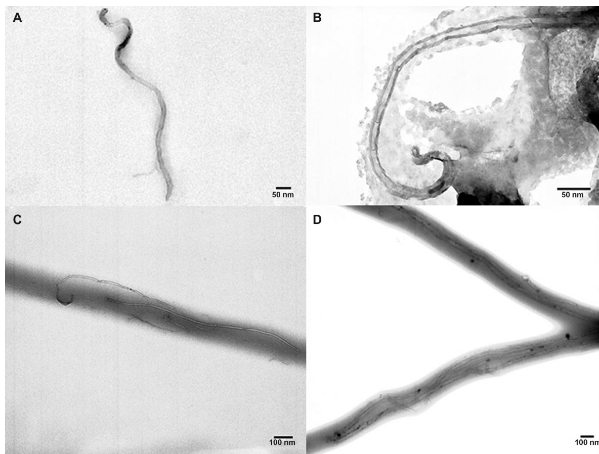
Figure 3 Transmission electron microscopic images. Electrospun (A) SWNT, (B) MWNT, (C) SWNT-10PU, and (D) MWNT-10PU. Abbreviations: MWNT, multiwalled nanotubes; SWNT, single-walled nanotubes; 10PU, 10% w/v polyurethane.
