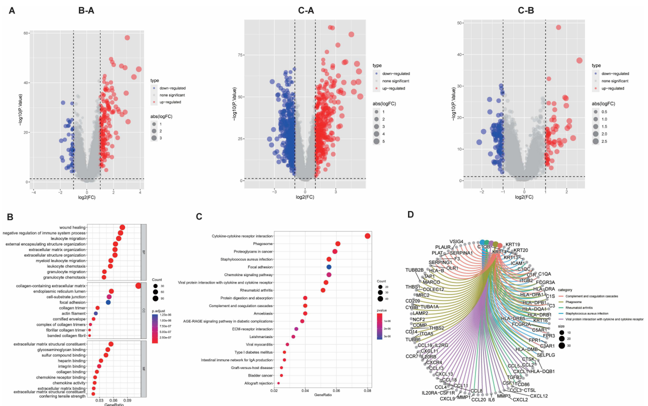
Figure 9 Recognition and functional enrichment analysis of DEGs among tumor subtypes. (A) Volcano plot of DEGs between clusters (A-C) . (B) Bubble plots of the GO terms of DEGs. (C) Bubble plots of the KEGG pathways of DEGs. (D) Counterparts of top 5 pathway and genes in KEGG enrichment analysis.
