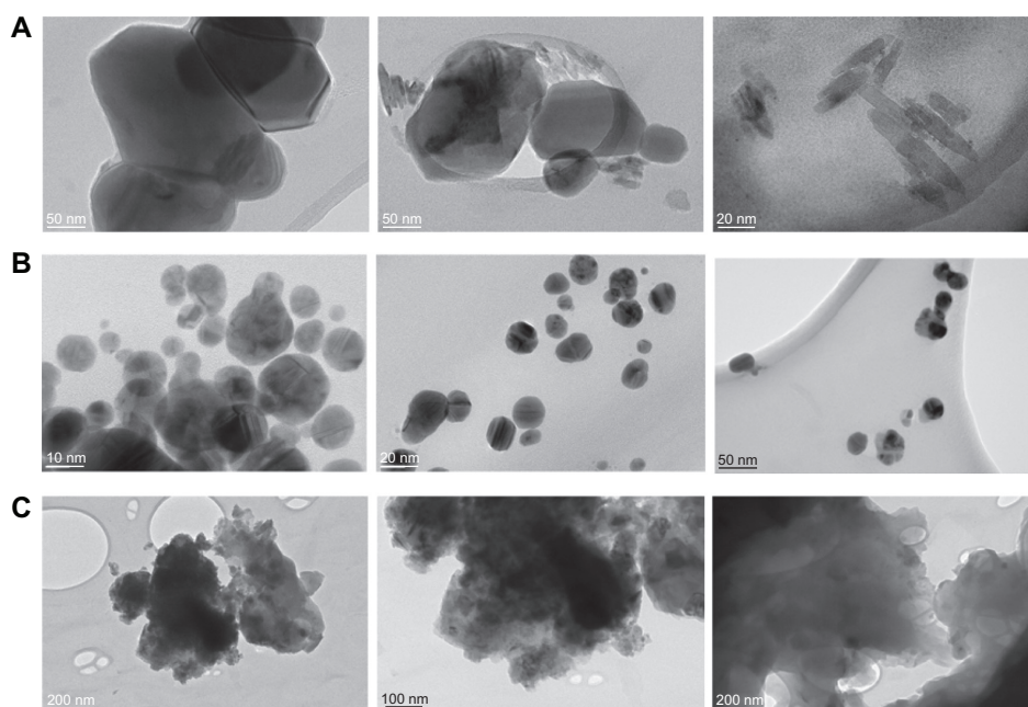
Figure 4 TEM images of bare silver nanoparticles (A), capped with 0.1% PGA (B) and with 0.4% PGA (C). Abbreviations: TEM, transmission electron microscope; PGA, poly- \alpha , \gamma , L-glutamic acid.
