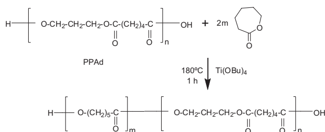
Figure 1 Schematic presentation of the chemical reactions during the preparation of poly(propylene adipate)-block-poly( \epsilon -caprolactone) copolymers.
