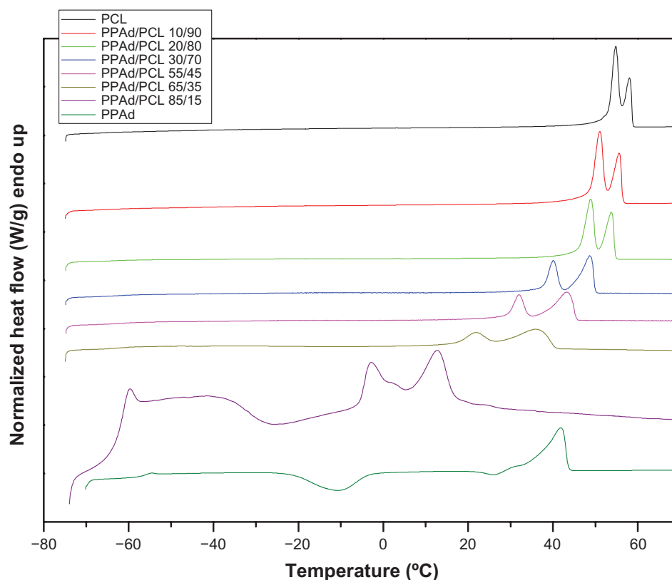
Figure 5 Differential scanning calorimetric thermograms of neat polymers and synthesized copolymers.
