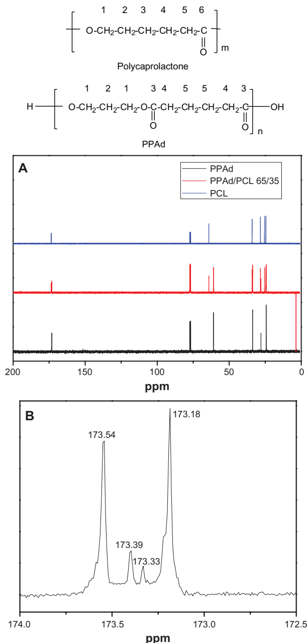
Figure 3 Carbon-13 nuclear magnetic resonance ( 13 C NMR) spectrum of poly(ε-caprolactone) (PCL), poly(propylene adipate) (PPAd), and their copolymer PPAAd/PCL 65/35 weight/weight (A) and 13 C-NMR spectrum at region 173 ppm of PPAAd/PCL 65/35 weight/weight (B).
