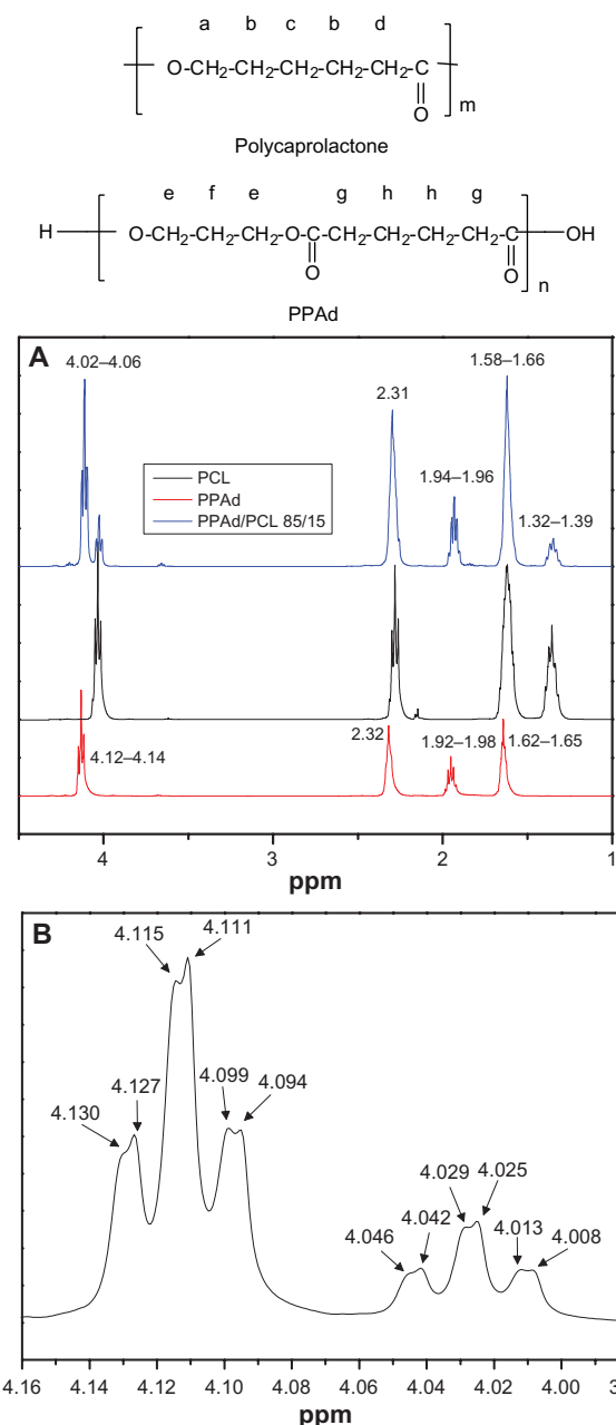
Figure 2 Hydrogen-1 nuclear magnetic resonance ( 1 H NMR) spectra of poly(ε-caprolactone) (PCL), poly(propylene adipate) (PPAd), and PPAAd/PCL 85/15 weight/weight copolymer (A) and 1 H NMR spectra of PPAAd/PCL 85/15 weight/weight copolymer at the region 3.98–4.16 ppm (B).
