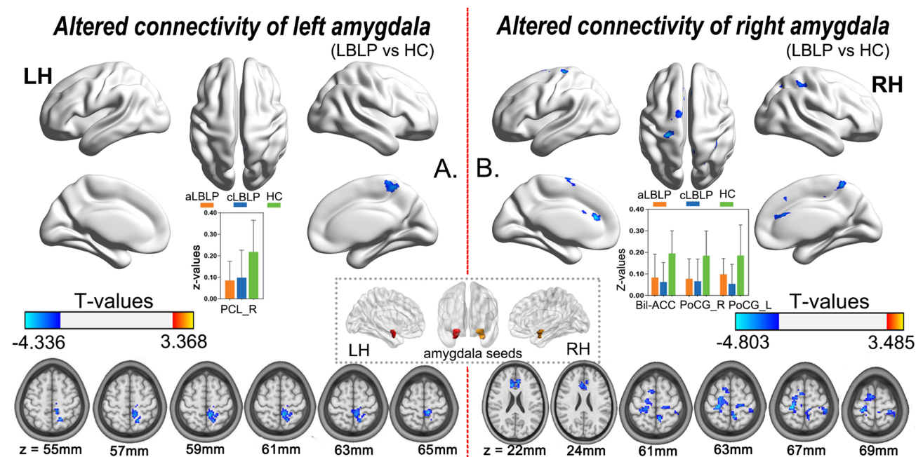
Figure 1 Altered connectivity of the left (A) and right (B) amygdala in LBLP patients (voxel-level P < 0.01 , GRF correction at cluster-level P < 0.05 ).
