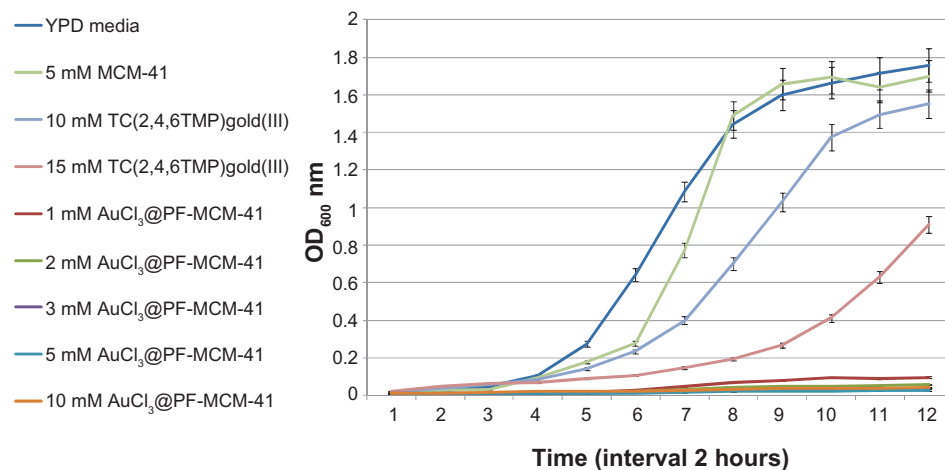
Figure 5 Growth curves of yeast cells by adding the moderate amounts of MCM-41, trichloro(2,4,6-trimethylpyridine)Au(III) and \text{AuCl}_3 @PF-MCM-41. The cells grew about control in YPD media under the condition of 5 mM MCM-41. Up to 15 mM TC(2,4,6TMP)gold(III) was tolerated. 1 mM was growth rate inhibition threshold for \text{AuCl}_3 @PF-MCM-41.
