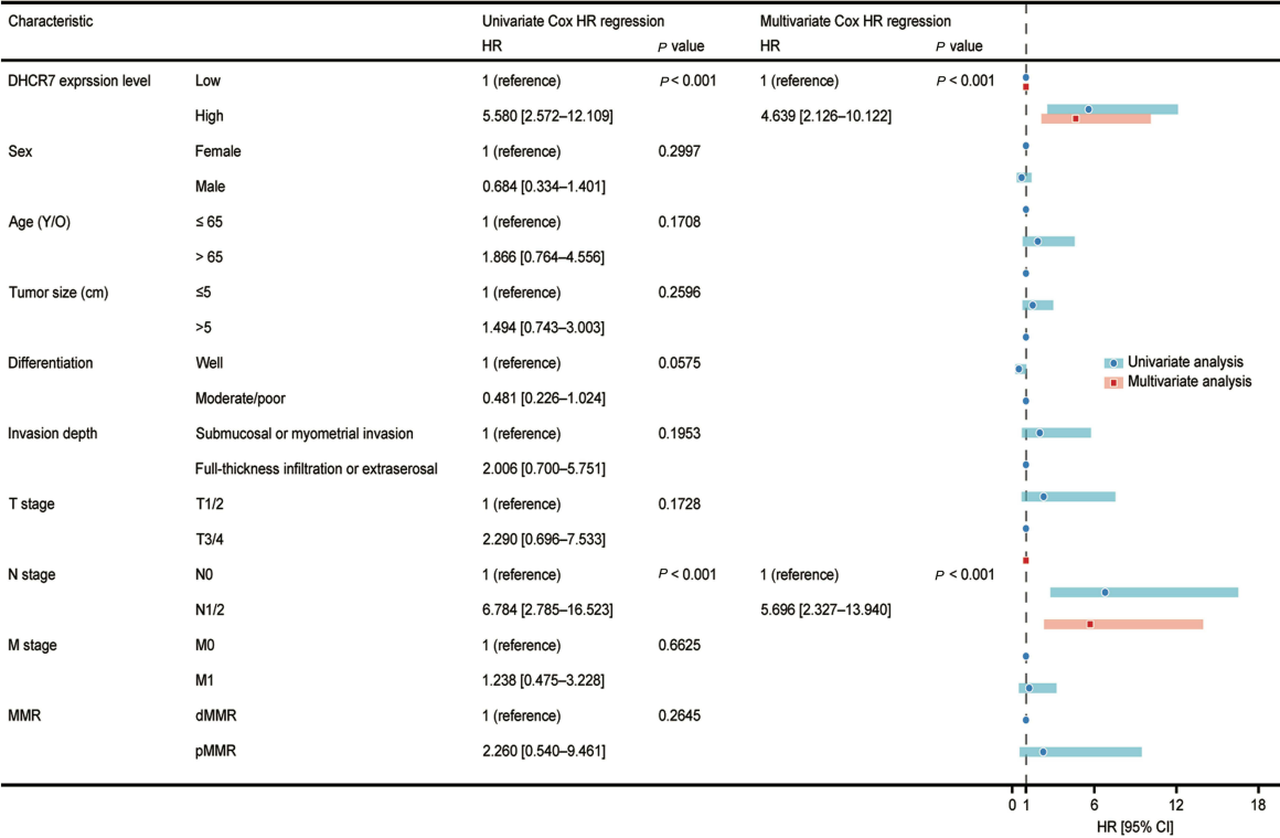
Figure 7 Survival analysis in relation to high and low expression of DHCR7 determined by immunohistochemistry in the CMU cohort (A) Kaplan–Meier survival curves for DHCR7. (B) Univariable and multivariable analyses of factors associated with overall survival.
