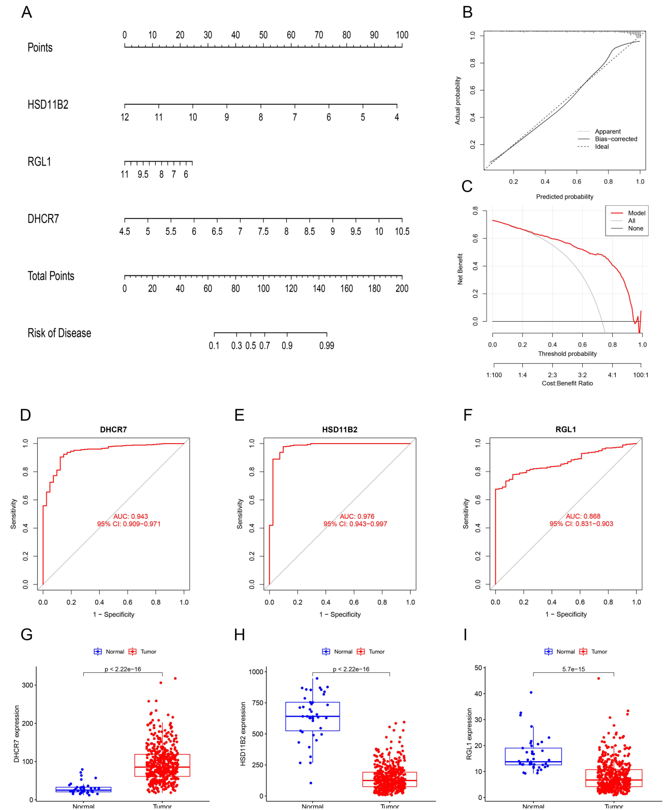
Figure 3 Generation and validation of the nomogram for colon cancer diagnosis. (A) Nomogram to predict the occurrence of colon cancer. (B) Calibration curve for evaluating the diagnostic performance and (C) decision curve for evaluating the clinical value of the nomogram. (D–F) ROC curves for DHCR7 , HSD11B2 , and RGL1 . (G–I) Difference boxplots for DHCR7 , HSD11B2 , and RGL1 expression between normal and tumour samples.
