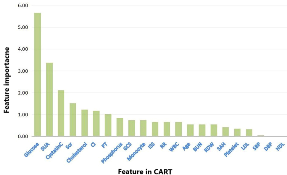
Figure 3 Feature importance of variables recognized by CART analysis.
