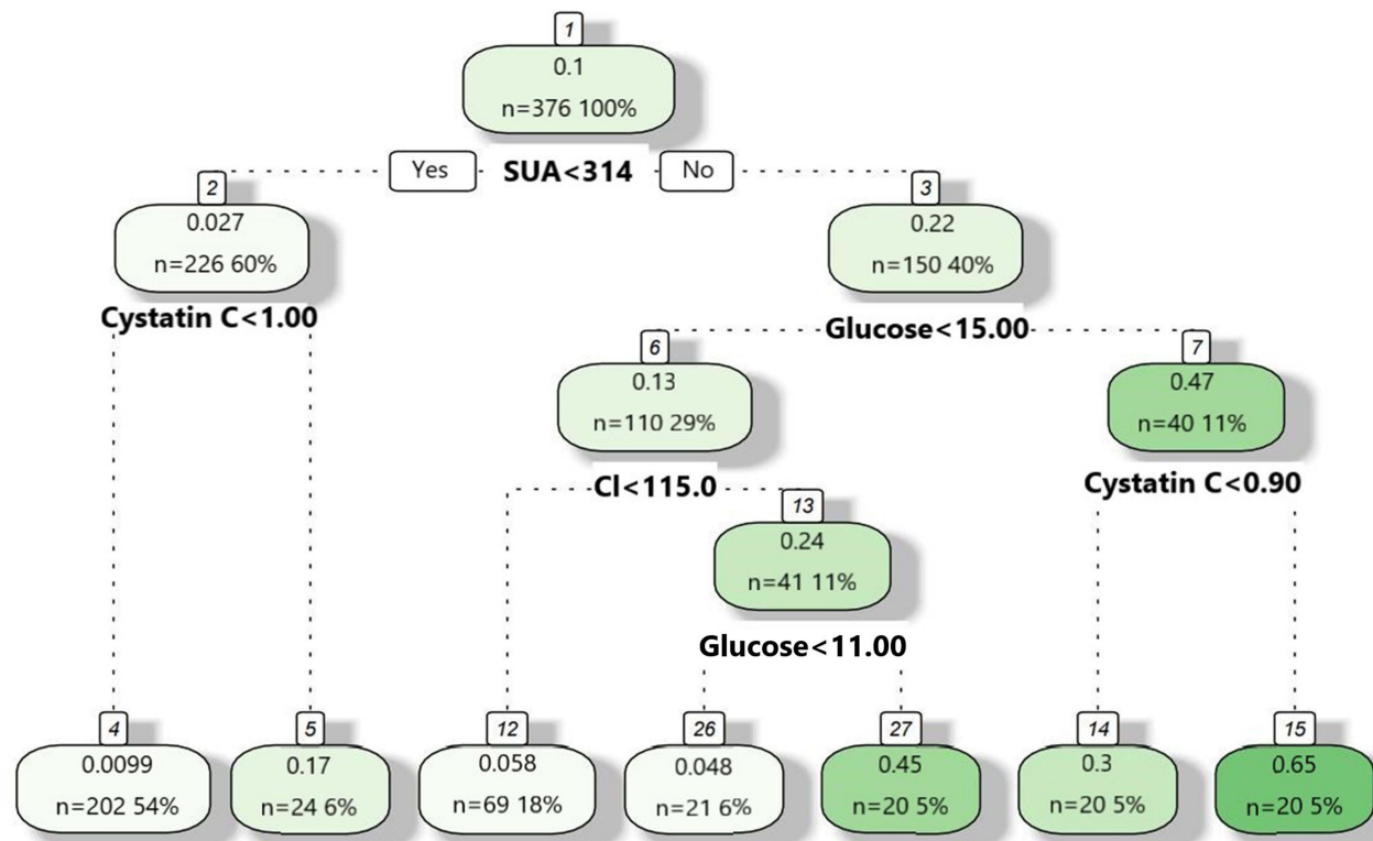
Figure 2 Decision tree model for the prediction of AKI in included TBI patients using CART analysis.
