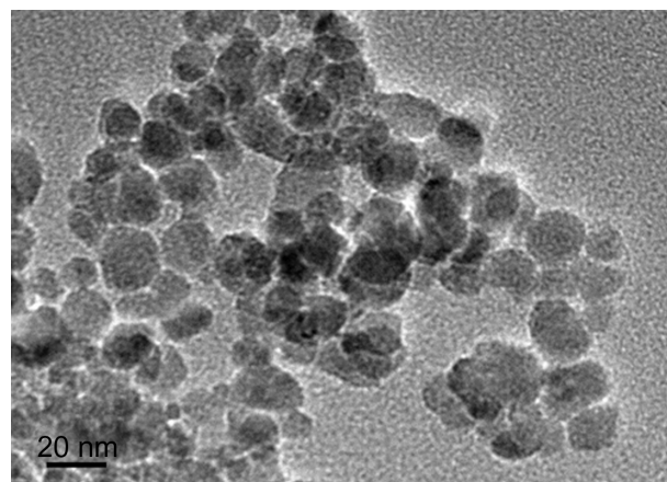
Figure 1 Transmission electron microscope image of magnetic \text{Fe}_3\text{O}_4 nanoparticles.
