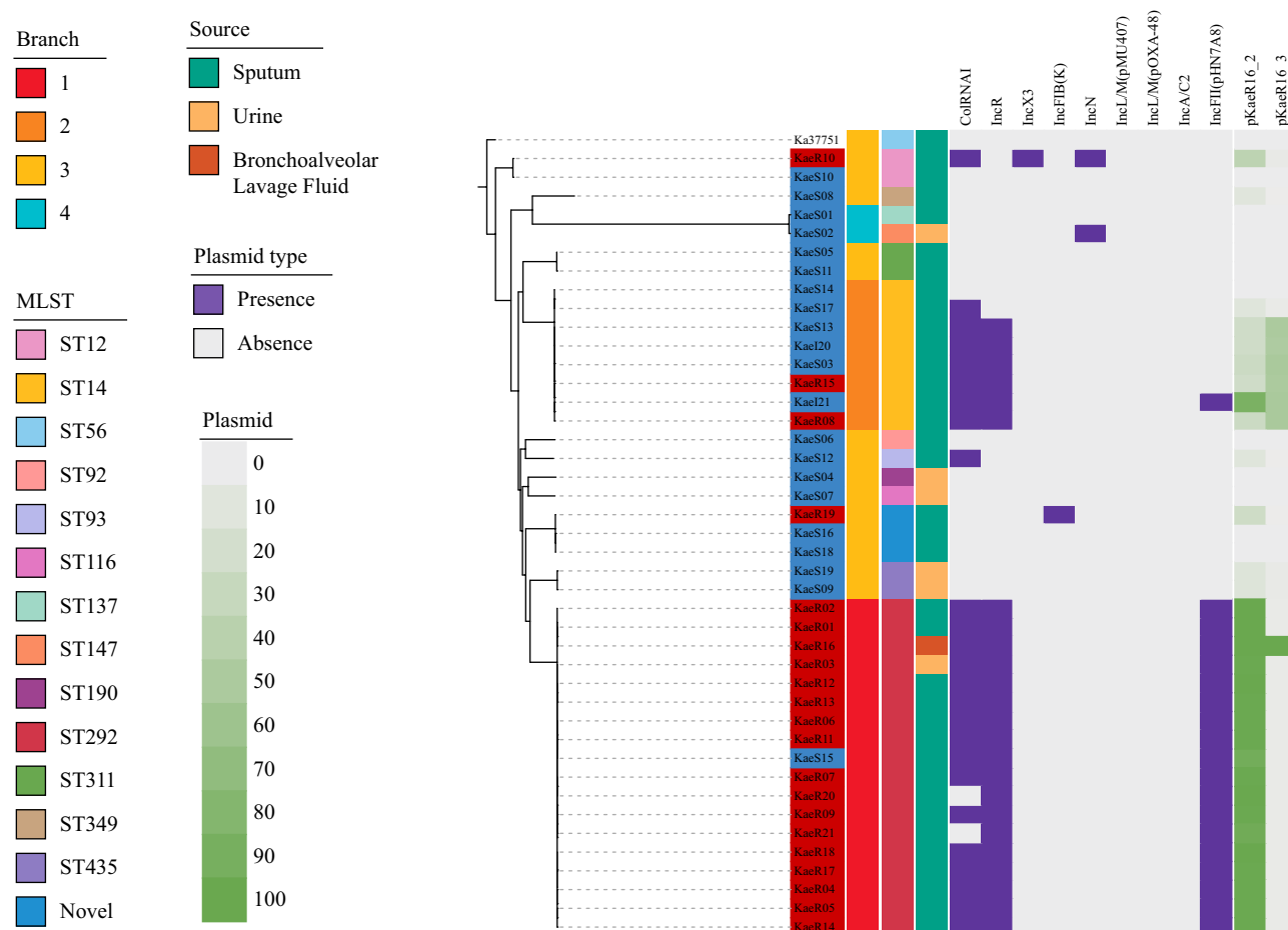
Figure 3 The plasmid replicons and the distribution of pKaeR16-2 and pKaeR16-3 in the K. aerogenes strains.
