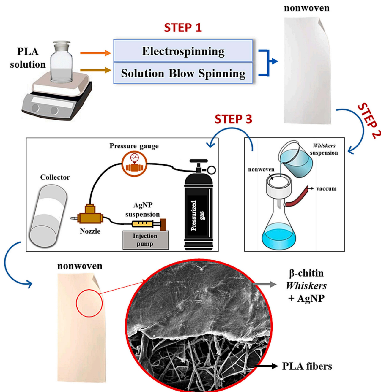
Figure 7 Schematic of the production method of bilayer membranes.
