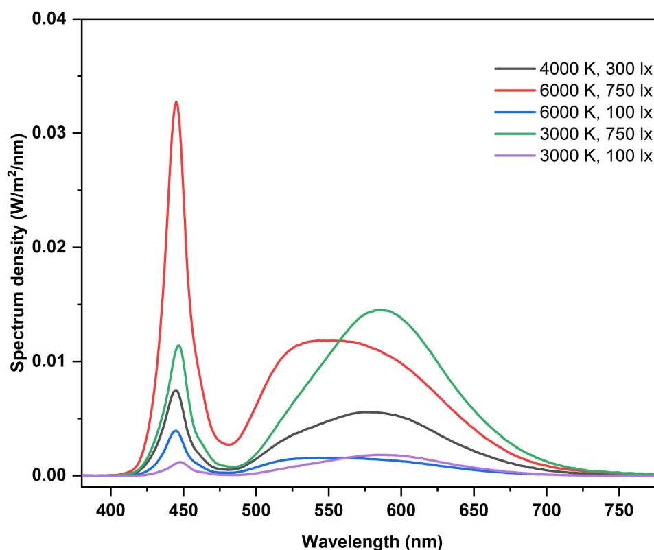
Figure 1 Spectrum power distribution measured at eye level for one baseline (300 lx, 4000 K) and four light exposure intervention settings.
