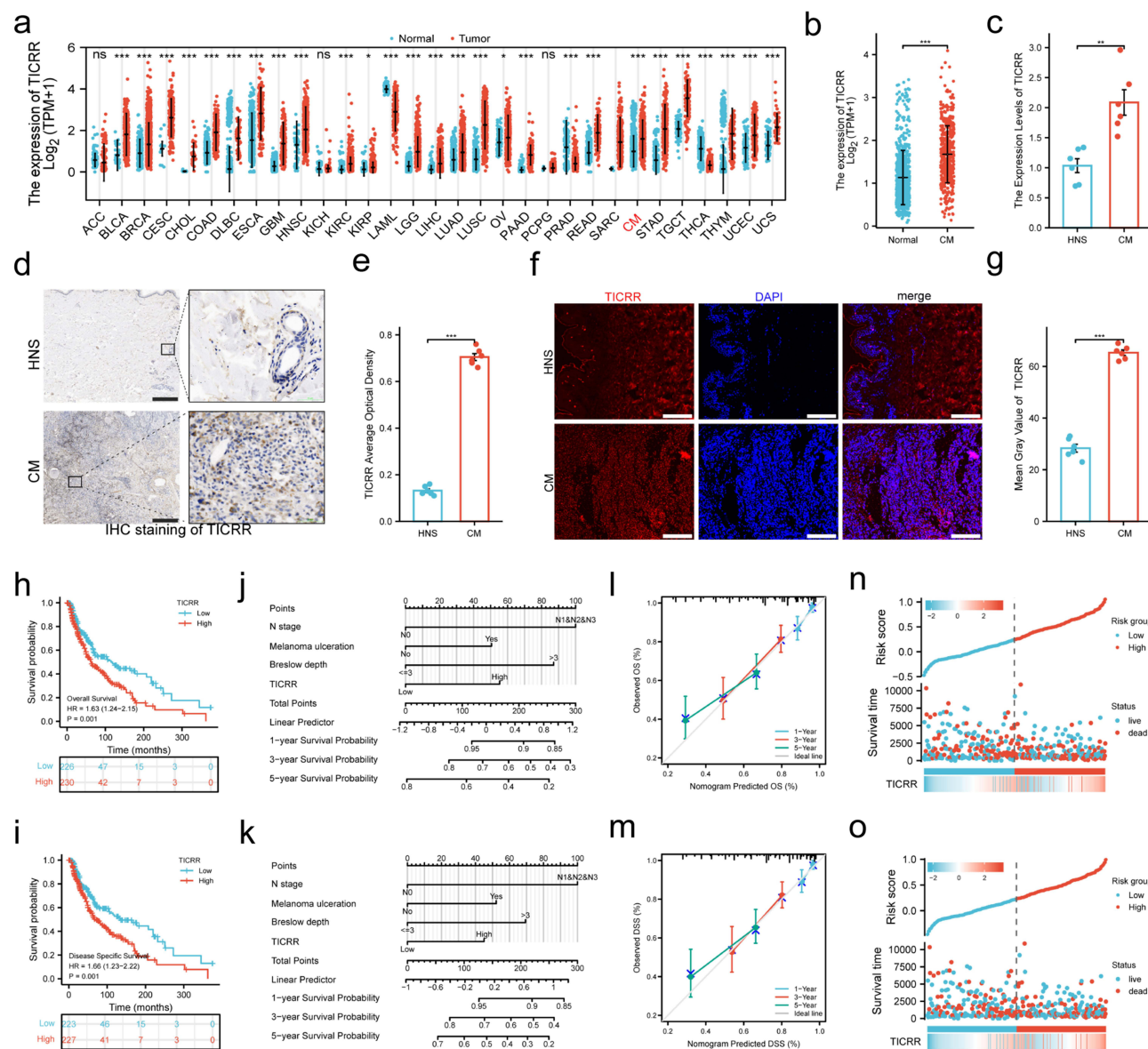
Figure 1 TICRR was overexpressed in CM and associated with worse prognostic value. (a) TICRR was highly expressed in most cancer species, including CM. (b) Comparison of mRNA levels of TICRR in CM and HNS tissues from TCGA and GTEx databases. (c) mRNA levels of TICRR in collected samples ( n = 6 ). (d and e) Representative images of TICRR immunohistochemistry and corresponding quantification in collected CM and HNS tissues ( n = 6 ; scale bar = 500 \mu m). (f and g) Representative pictures of TICRR immunofluorescence and corresponding quantification in collected CM and HNS tissues ( n = 6 ; scale bar = 200 \mu m). (h and i) Kaplan-Meier analysis of OS (h) and DSS (i) in CM patients with different TICRR expression levels. (j and k) Nomogram model predicting the 1-year, 3-year, 5-year OS (j) and DSS (k) of patients with CM. (l and m) Calibration chart evaluating the predictive accuracy of the nomogram. (n and o) Risk score curve showing TICRR expression, OS status (n) , DSS status (o) , and risk score. ns, P \geq 0.05 ; *, P < 0.01 ; ***, P < 0.001 .
