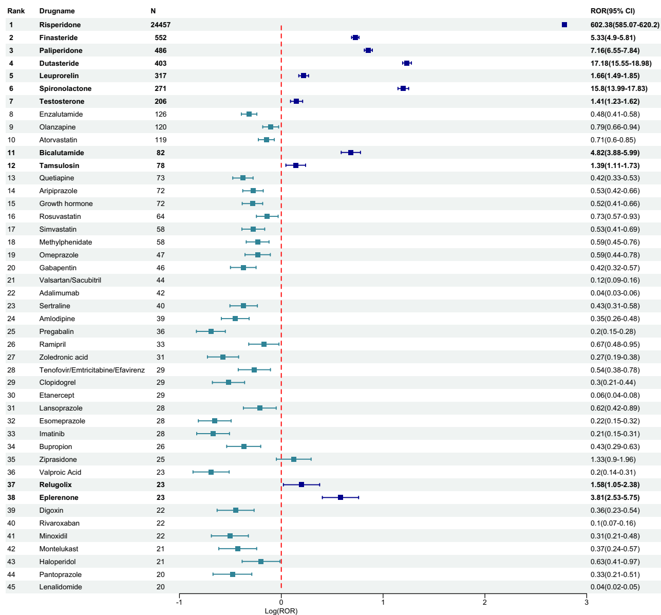
Figure 3 Forest plot of Reporting Odds Ratios for the Top 45 Drugs Causing Gynecomastia.
