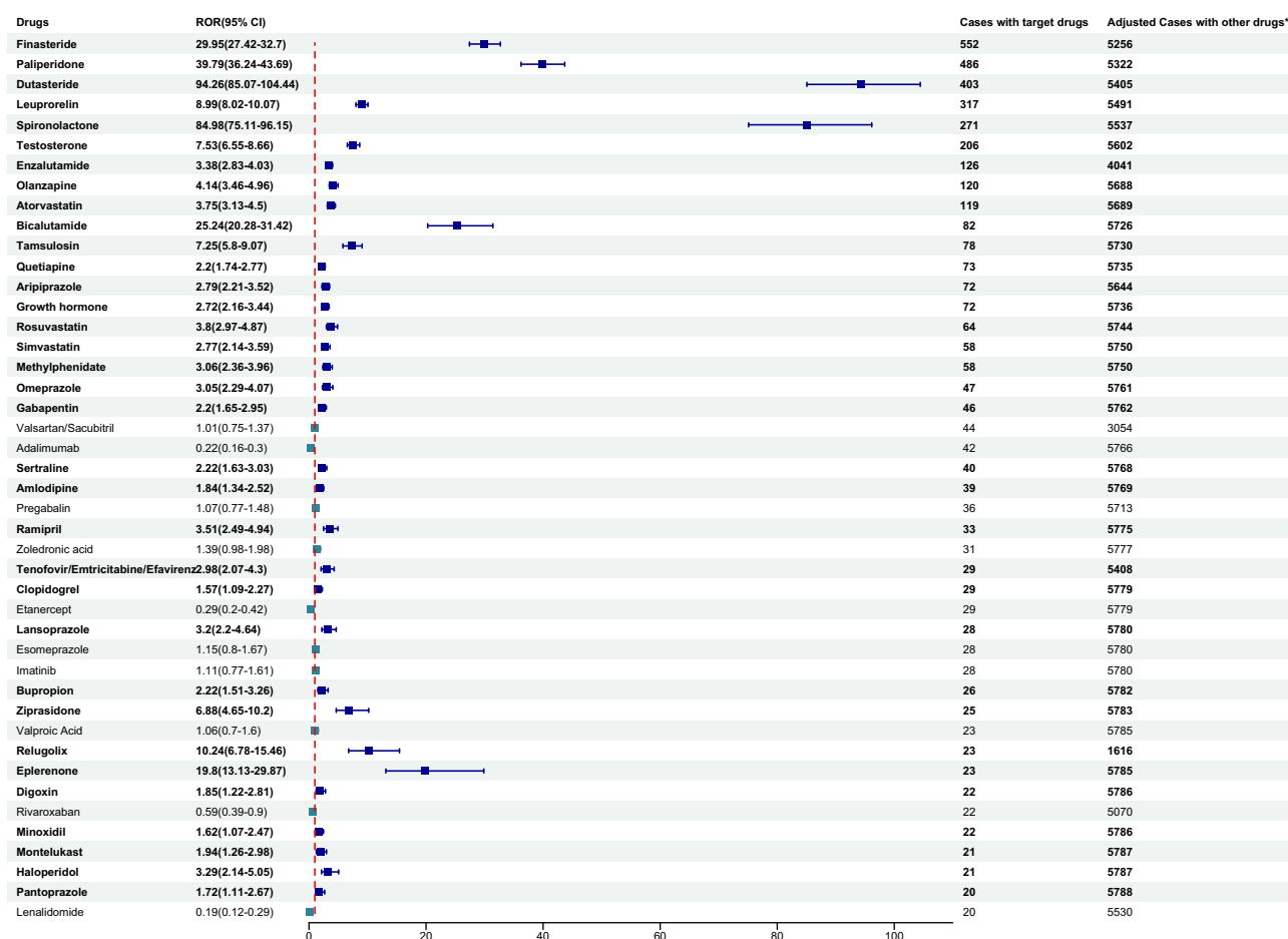
Figure 4 Forest plot of Sensitivity Analysis of Reporting Odds Ratios for the Top 2–45 Drugs Causing Gynecomastia.
