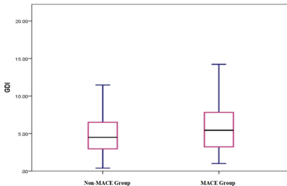
Figure 2 Comparison of GDI Values between Non-MACE Group and MACE Group.
