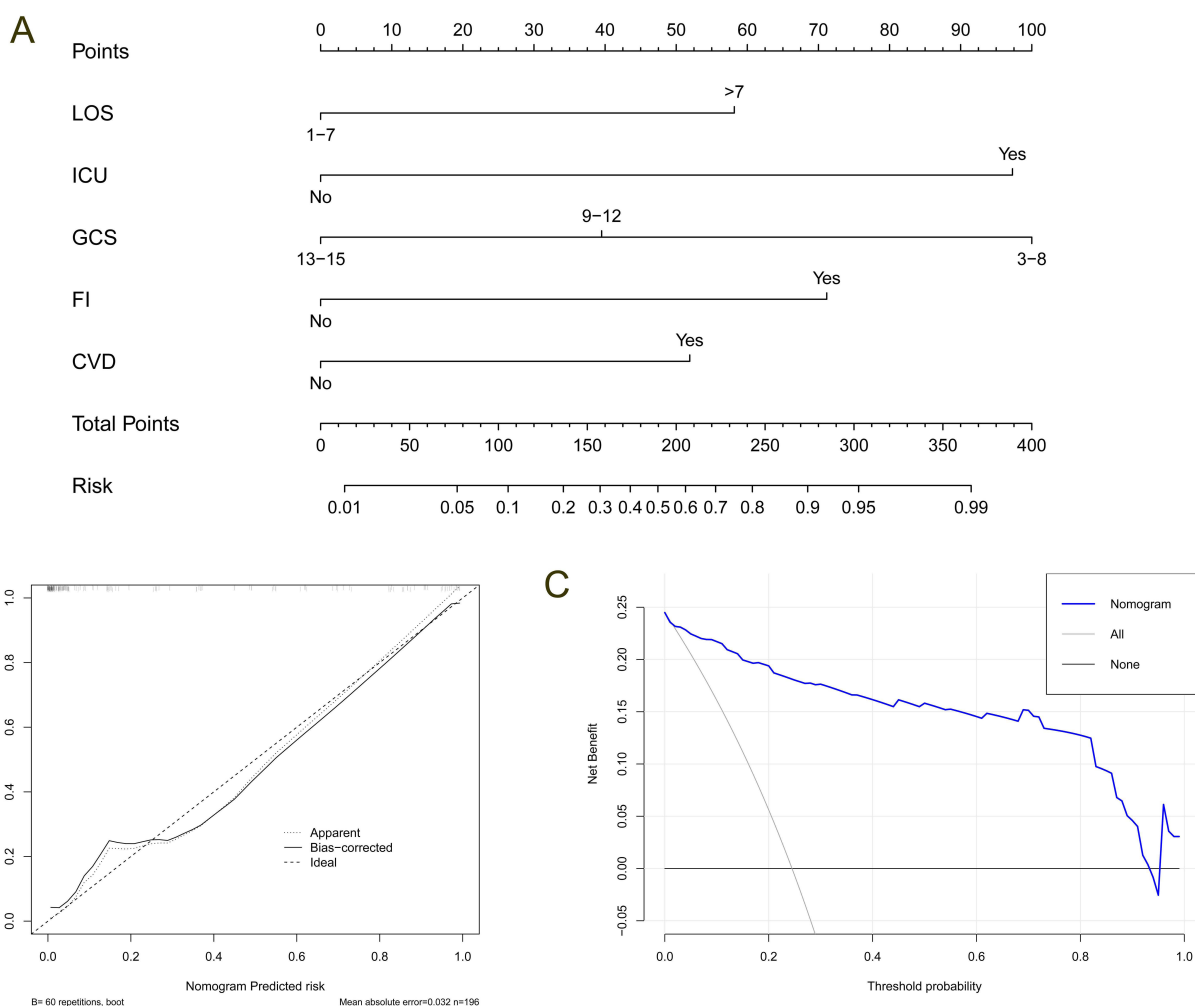
Figure 2 Nomogram. (A) Nomogram construction. (B) Calibration curve. (C) Decision curve.
