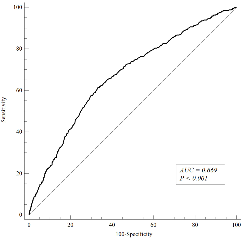
Figure 2 ROC curves of SUA/Cr for MAFLD.
