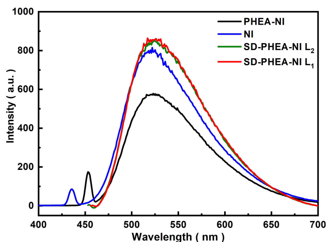
Figure 5 Fluorescent spectra of polyaspartamide fluorescent probes (SD-PHEA-NI).
